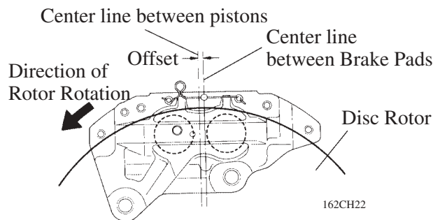
Brake Pad Offset and Installation
