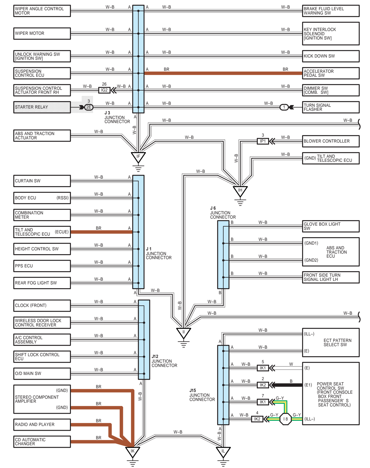
507 CENTURY (EWD366F)
