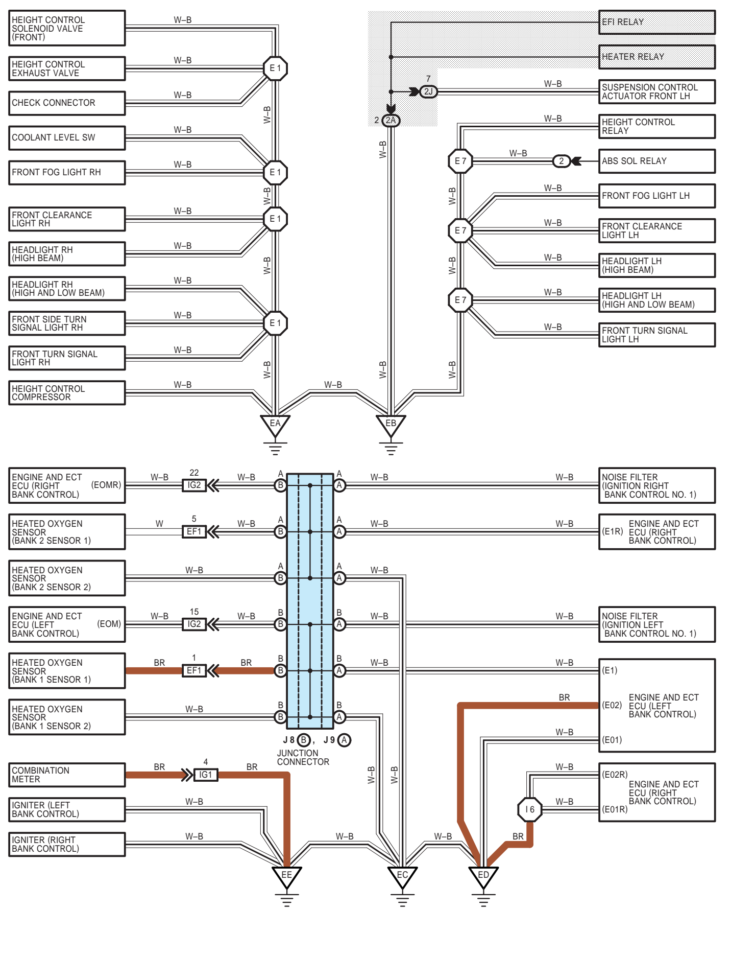
506 CENTURY (EWD366F)
