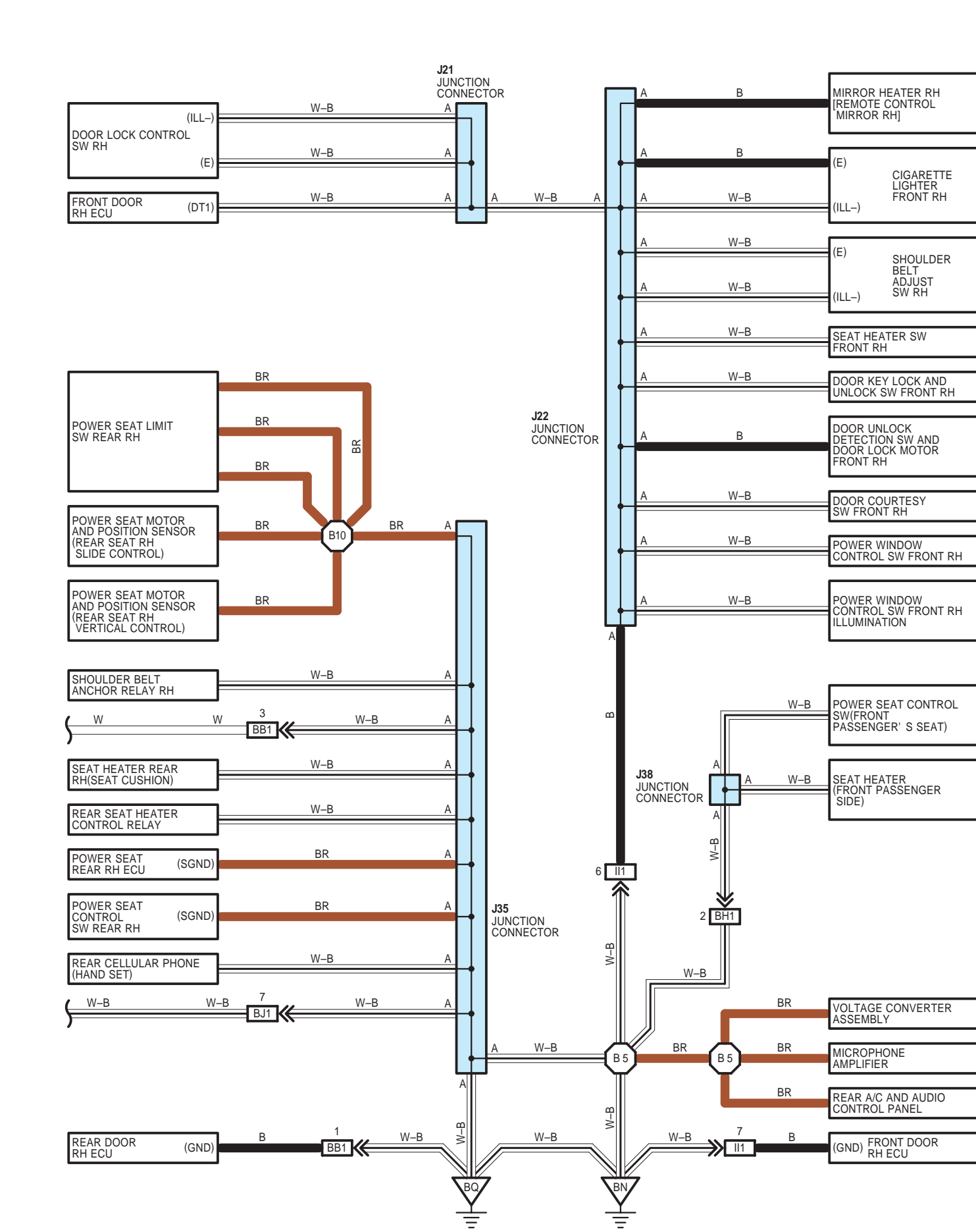
511 CENTURY (EWD366F)
