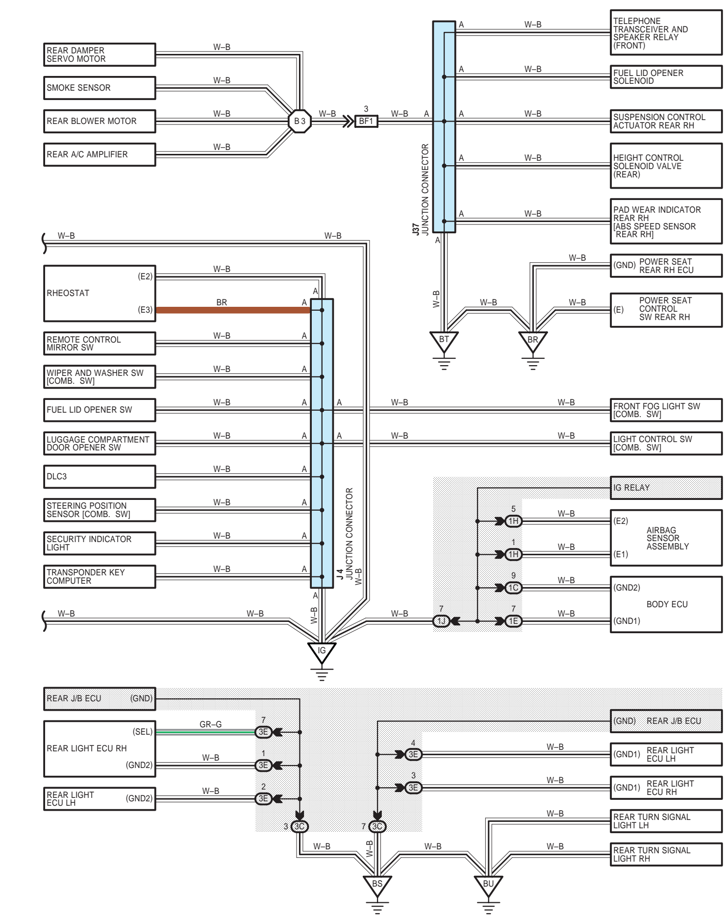
508 CENTURY (EWD366F)
