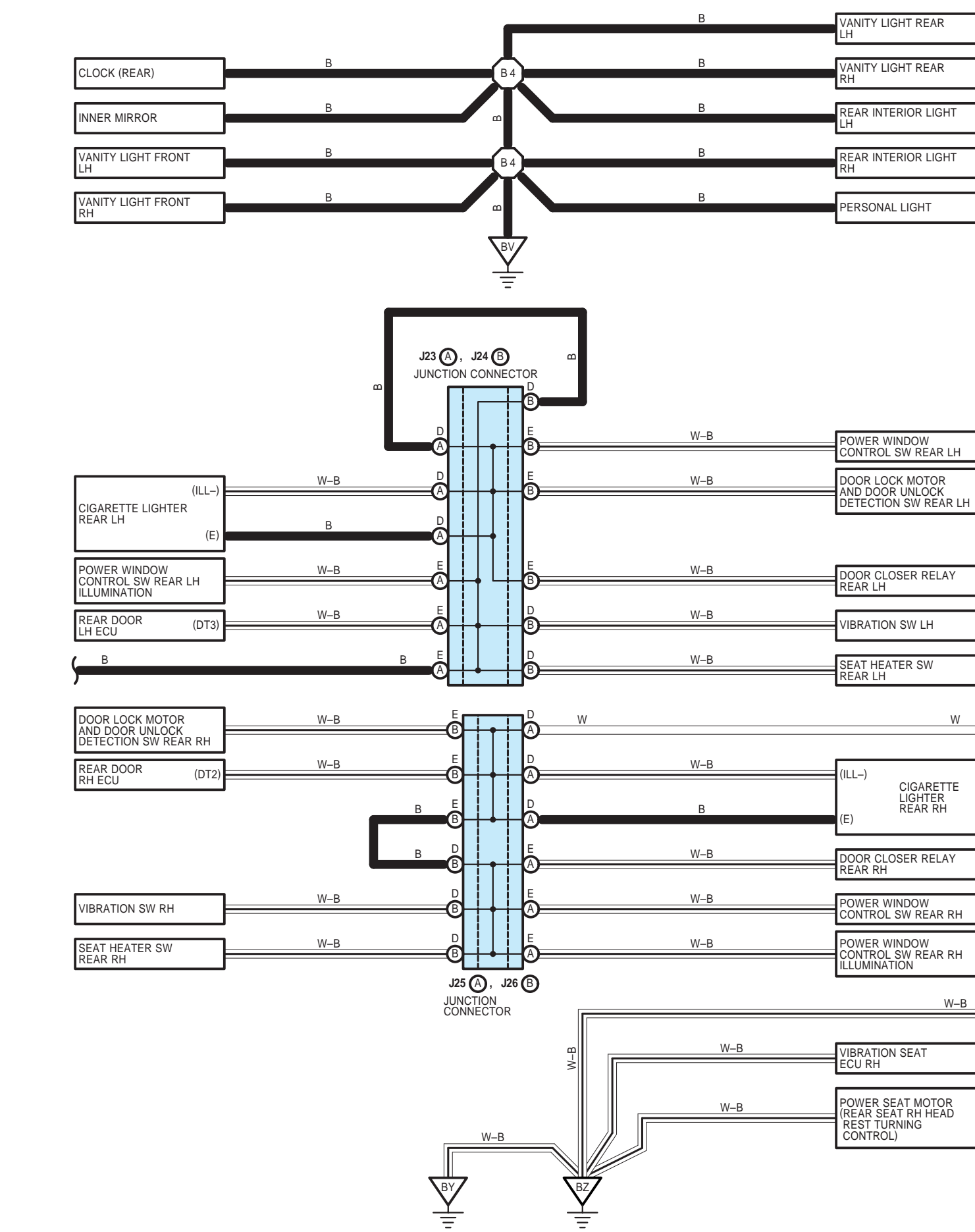
510 CENTURY (EWD366F)
