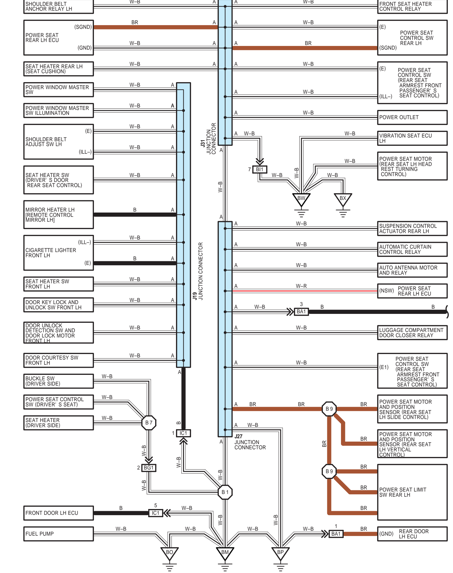
509 CENTURY (EWD366F)
