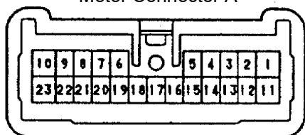
Meter Connector A
