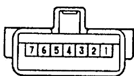
Meter Connector B
