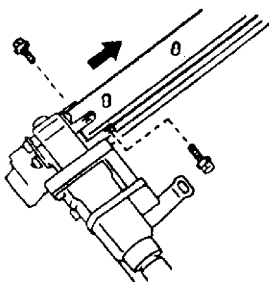
⑥ -1 Power seat motor (for slide)
