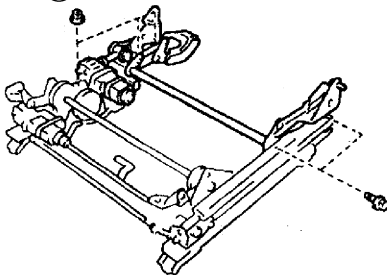
④ Front vertical adjuster
