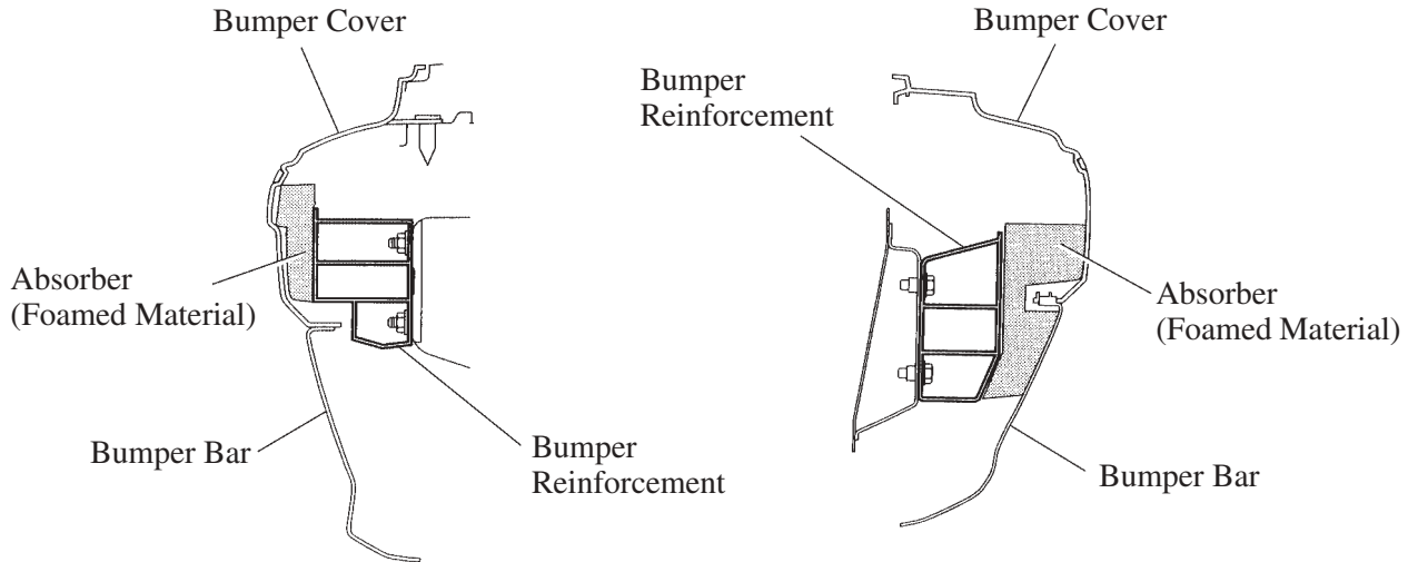
Front Bumper Cross Section
